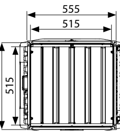
LEO L1 | L2 | L3 + KM L / LEO L1 BMS | L2 BMS | L3 BMS + KM L
