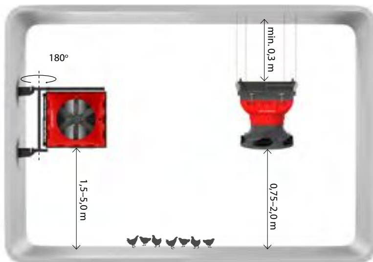
installation under the ceiling (1)
